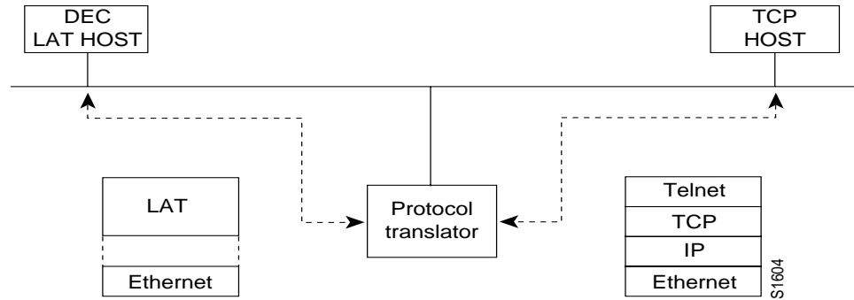
Figure 1-1 Comparing LAT and Telnet Protocol Stacks
